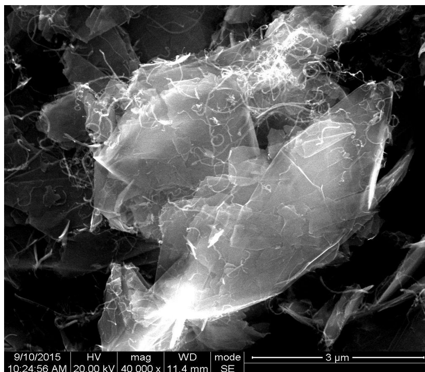
SEM of Graphite Nanoplatelet Carbon Nanotubes Powder Composite
